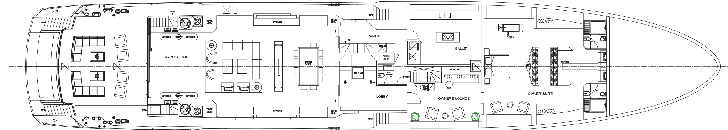
MAIN DECK
