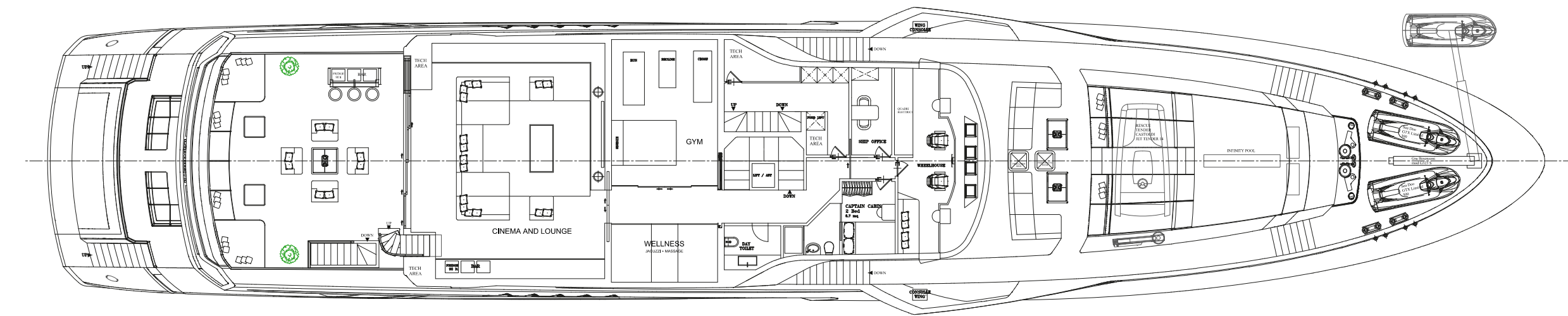
UPPER DECK
