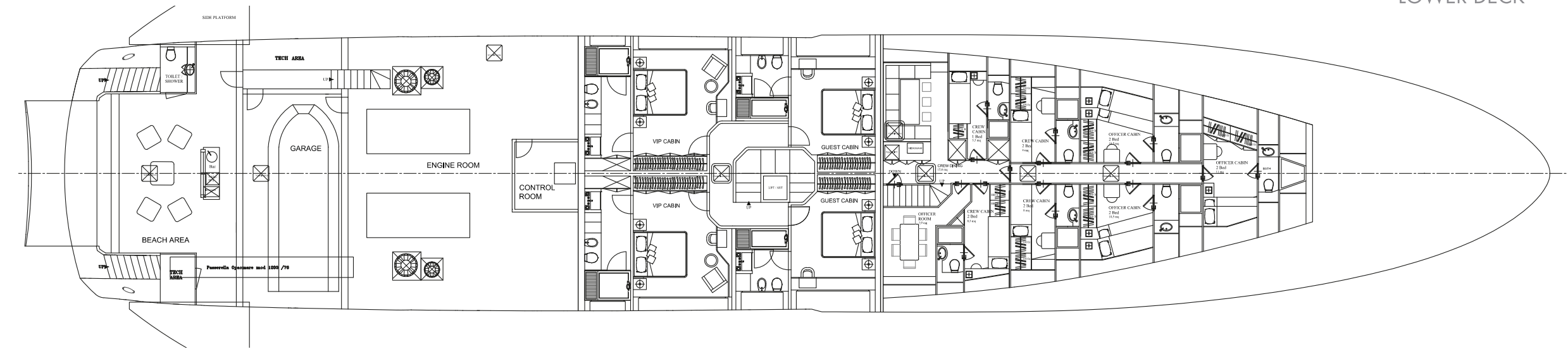
LOWER DECK
